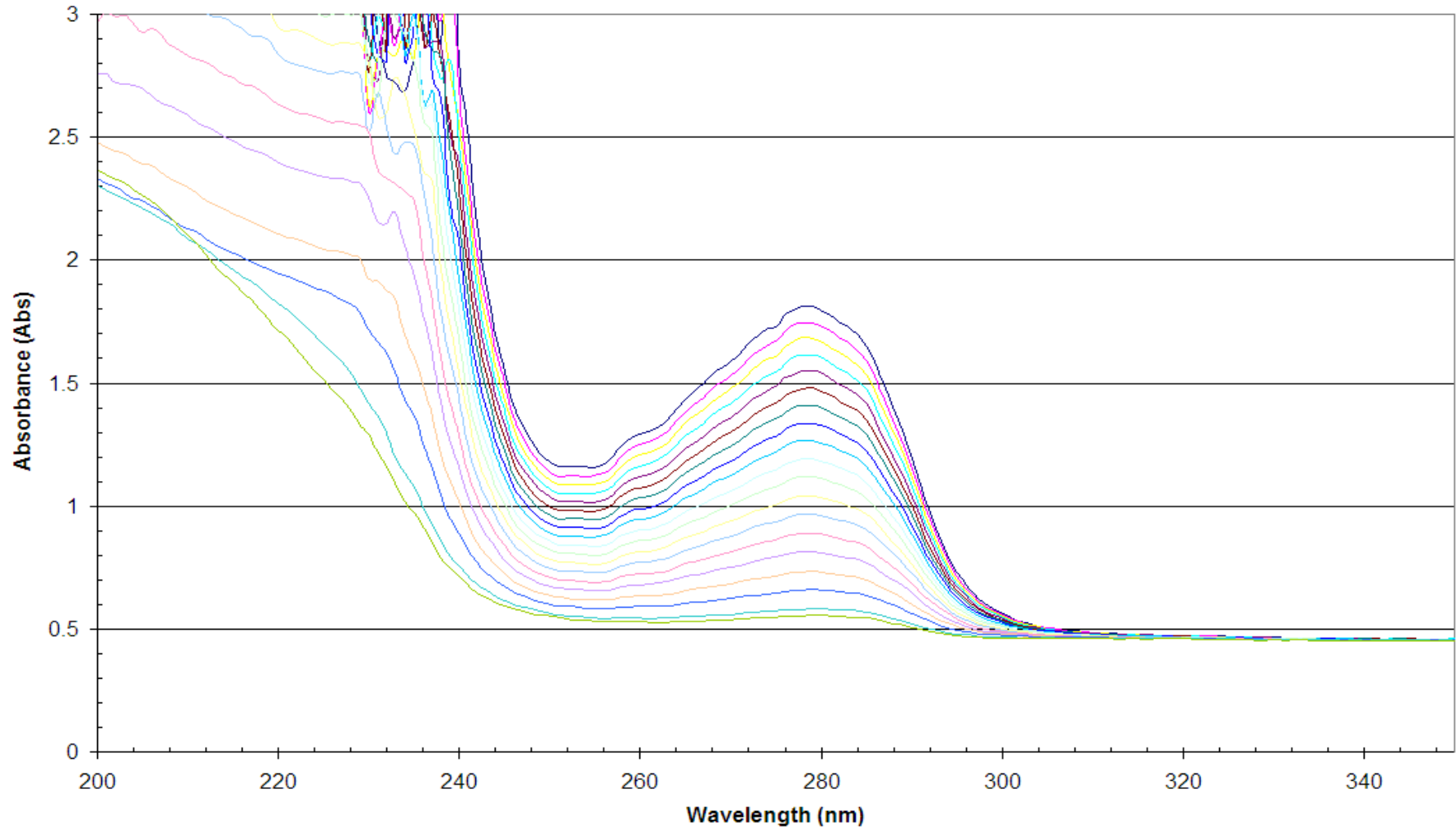
BSA - Concentration 220 mg/ml - Spectral Data at Various Pathlengths
