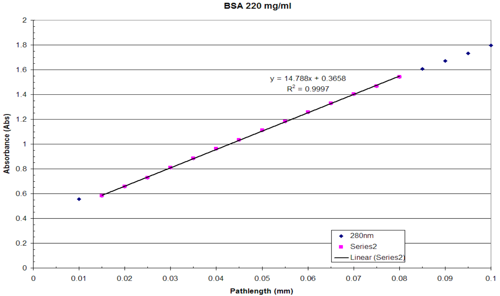
BSA - Concentration 220 mg/ml - Absorbance vs. Pathlength Linearity
