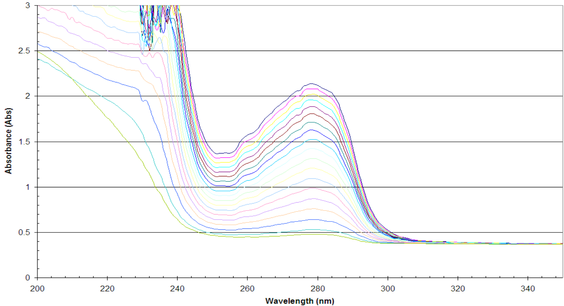
BSA - Concentration 300 mg/ml - Spectral Data at Various Pathlengths
