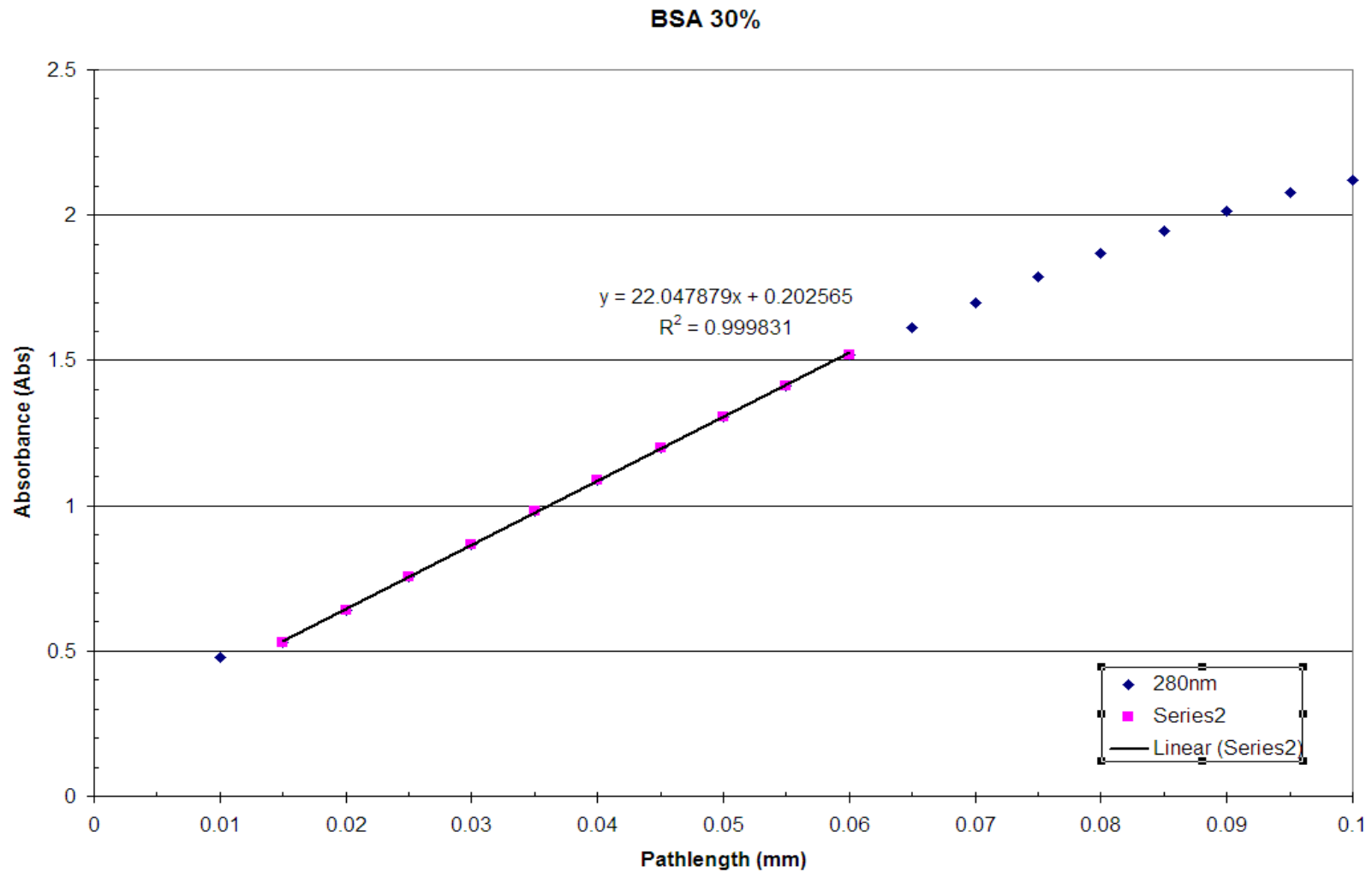
BSA - Concentration 300 mg/ml - Absorbance vs. Pathlength Linearity
